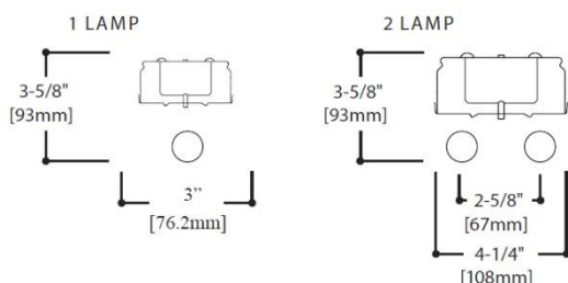
LAMP CONFIGURATION
